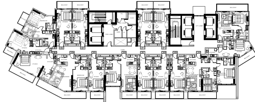
15th FLOOR
